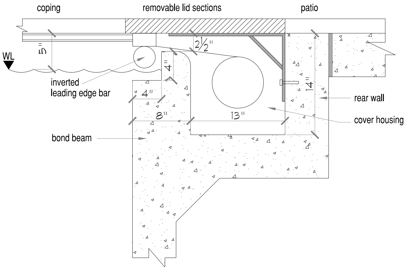
HIDDEN LEADING EDGE CROSS SECTION
